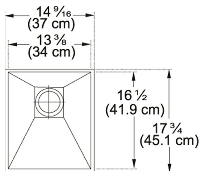
Technical Drawing
