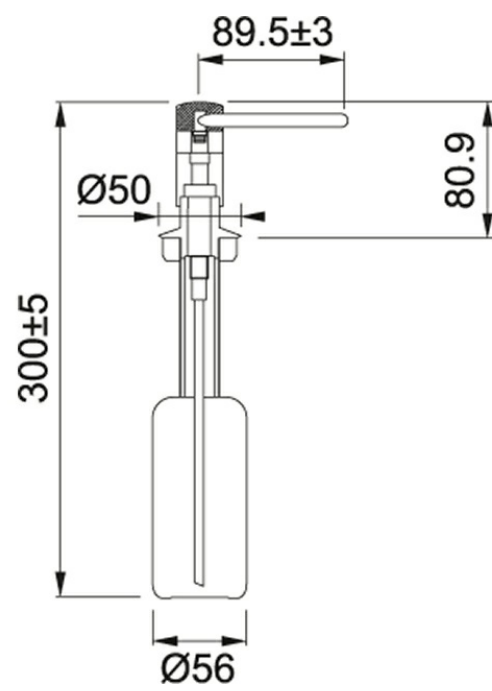
Technical Drawing
